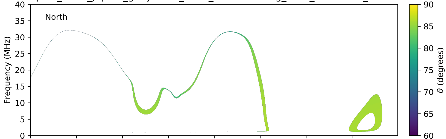
expres_earth_jupiter_ganymede_isaac_lossc-wid1deg_1kev_20160401_v01.cdf
