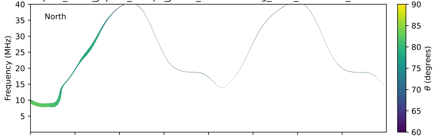
expres_earth_jupiter_europa_jrm33_lossc-wid1deg_3kev_20160426_v11.cdf
