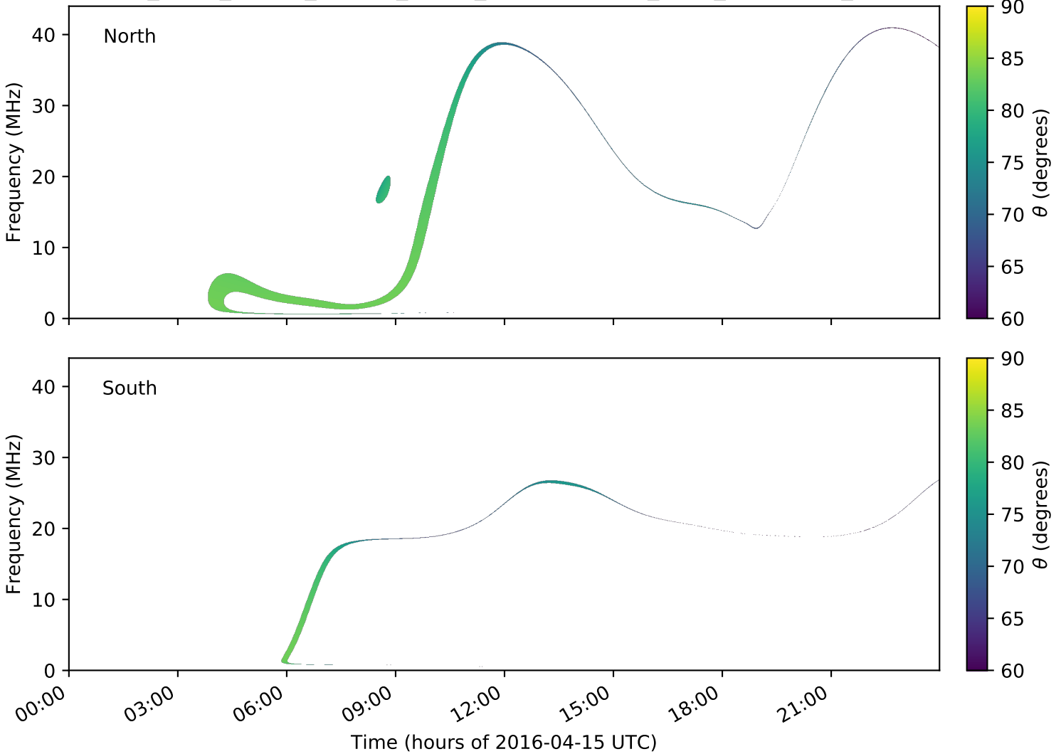
expres_earth_jupiter_europa_jrm09_lossc-wid1deg_3kev_20160415_v01.cdf
