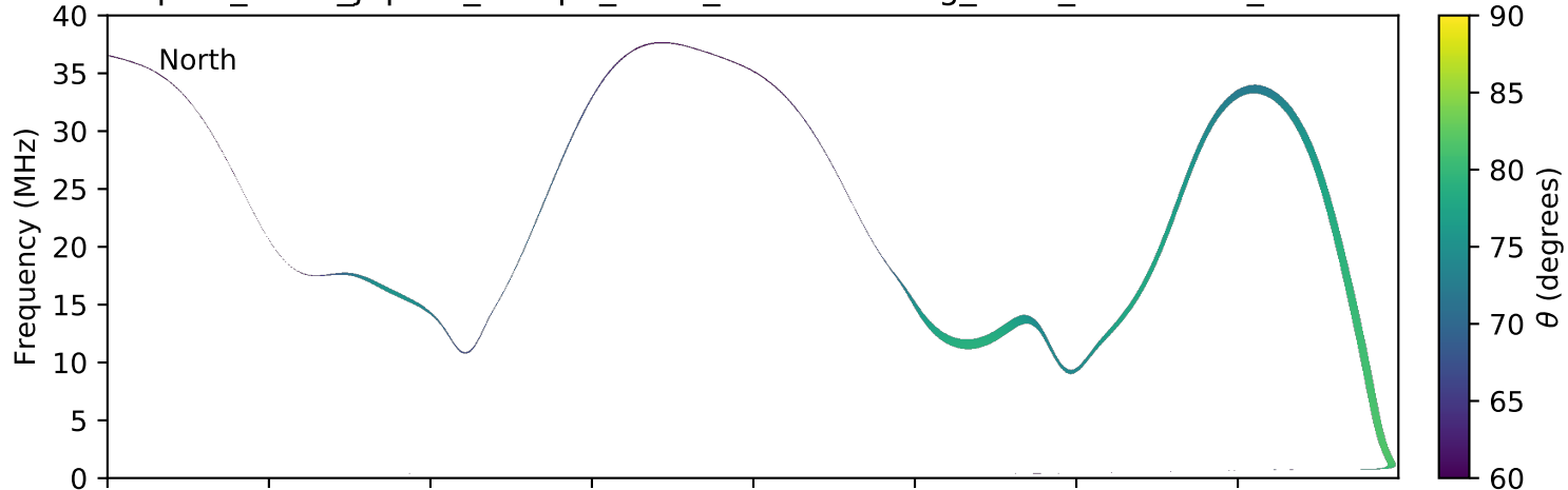
expres_earth_jupiter_europa_isaac_lossc-wid1deg_5kev_20160430_v01.cdf
