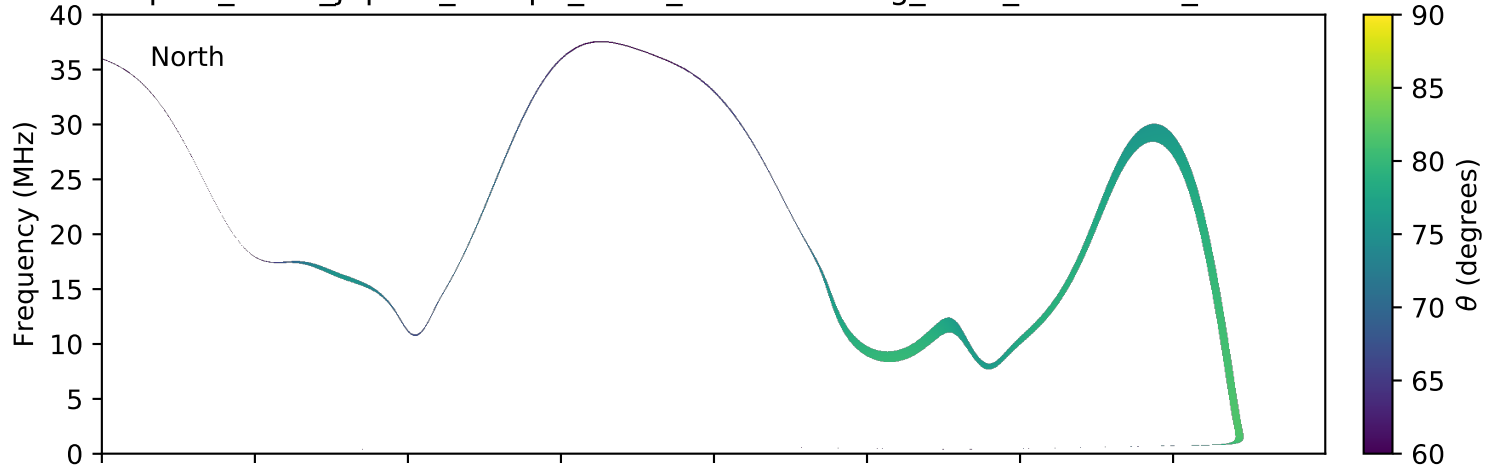
expres_earth_jupiter_europa_isaac_lossc-wid1deg_5kev_20160423_v01.cdf
