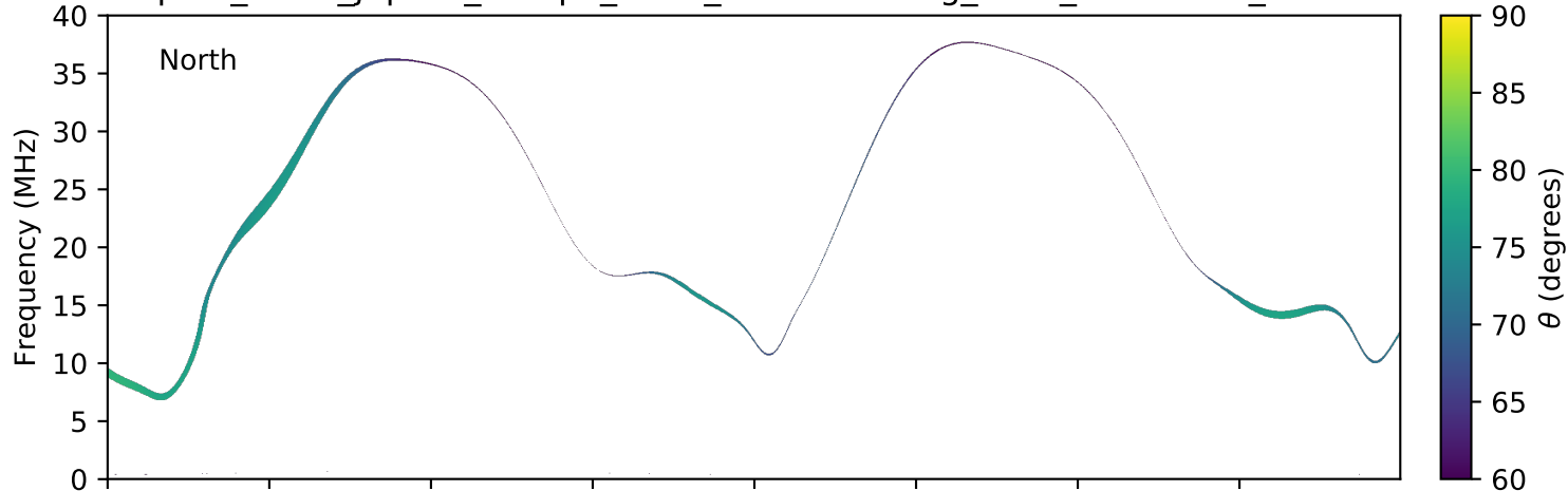
expres_earth_jupiter_europa_isaac_lossc-wid1deg_5kev_20160419_v01.cdf
