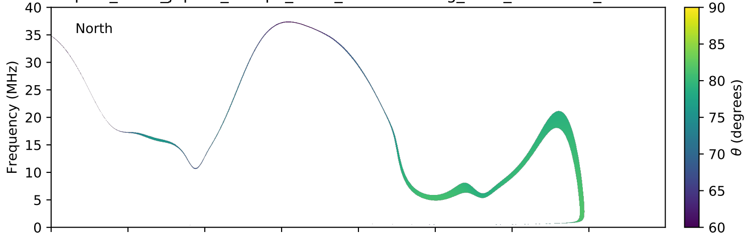
expres_earth_jupiter_europa_isaac_lossc-wid1deg_5kev_20160416_v01.cdf
