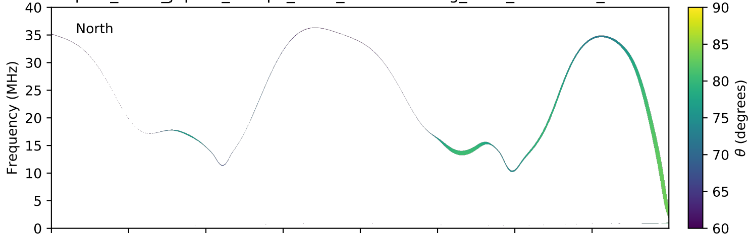
expres_earth_jupiter_europa_isaac_lossc-wid1deg_3kev_20160430_v01.cdf
