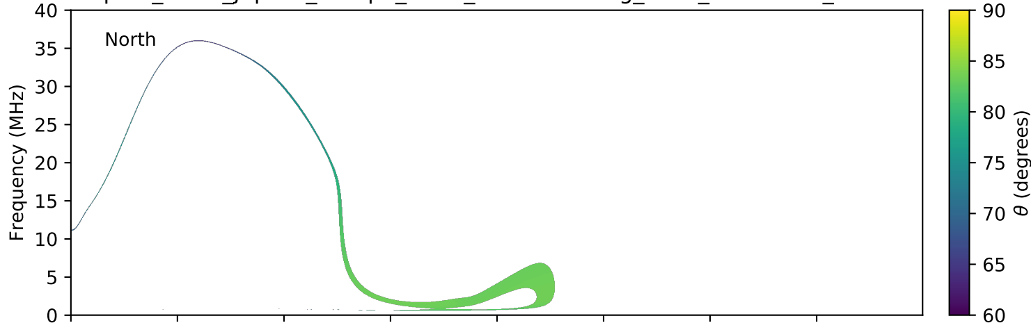
expres_earth_jupiter_europa_isaac_lossc-wid1deg_3kev_20160427_v01.cdf
