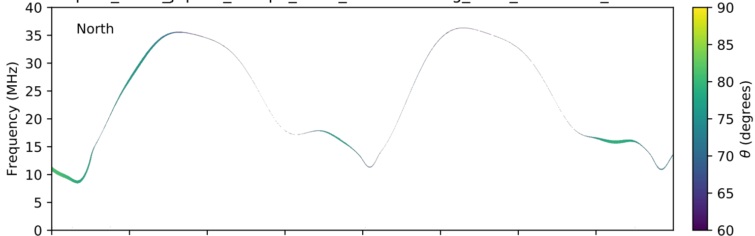
expres_earth_jupiter_europa_isaac_lossc-wid1deg_3kev_20160419_v01.cdf
