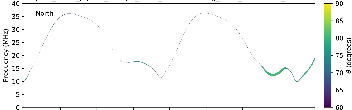
expres_earth_jupiter_europa_isaac_lossc-wid1deg_3kev_20160405_v01.cdf
