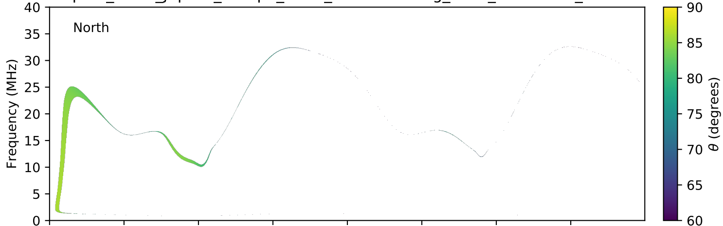
expres_earth_jupiter_europa_isaac_lossc-wid1deg_1kev_20160401_v01.cdf
