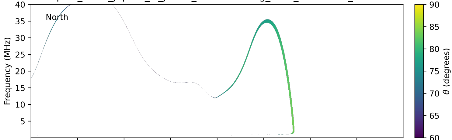
expres_earth_jupiter_io_jrm33_lossc-wid1deg_3kev_20160329_v11.cdf
