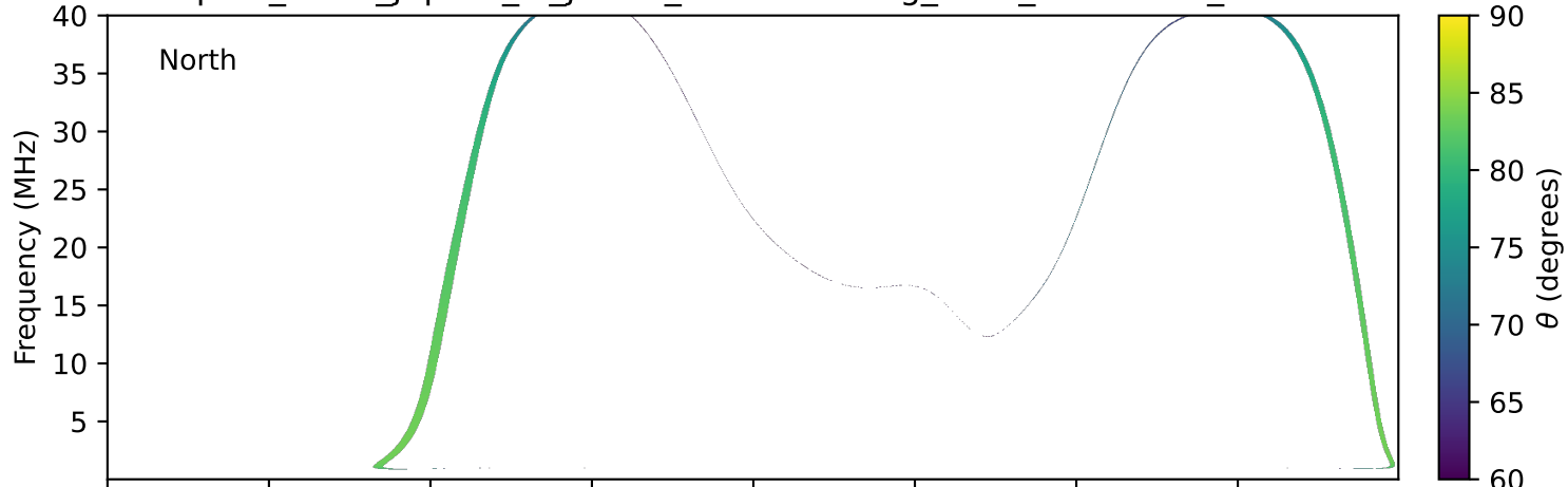
expres_earth_jupiter_io_jrm33_lossc-wid1deg_3kev_20160311_v11.cdf
