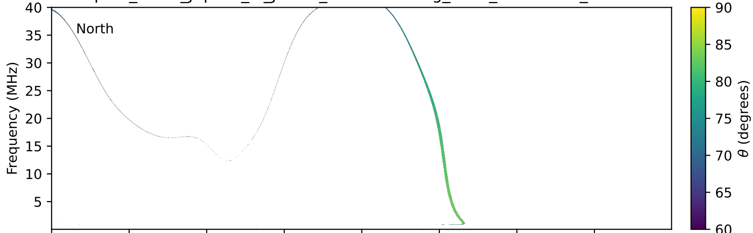
expres_earth_jupiter_io_jrm33_lossc-wid1deg_3kev_20160306_v11.cdf
