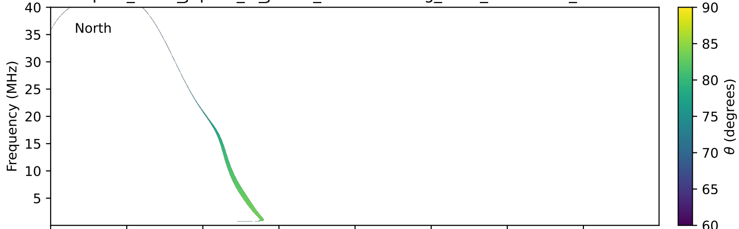
expres_earth_jupiter_io_jrm33_lossc-wid1deg_3kev_20160301_v11.cdf
