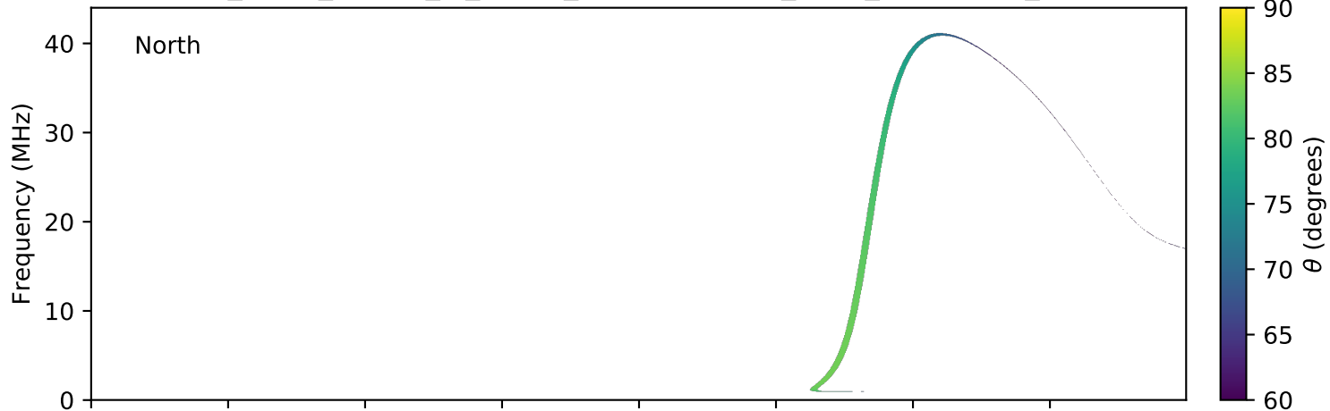
expres_earth_jupiter_io_jrm09_lossc-wid1deg_3kev_20160330_v01.cdf
