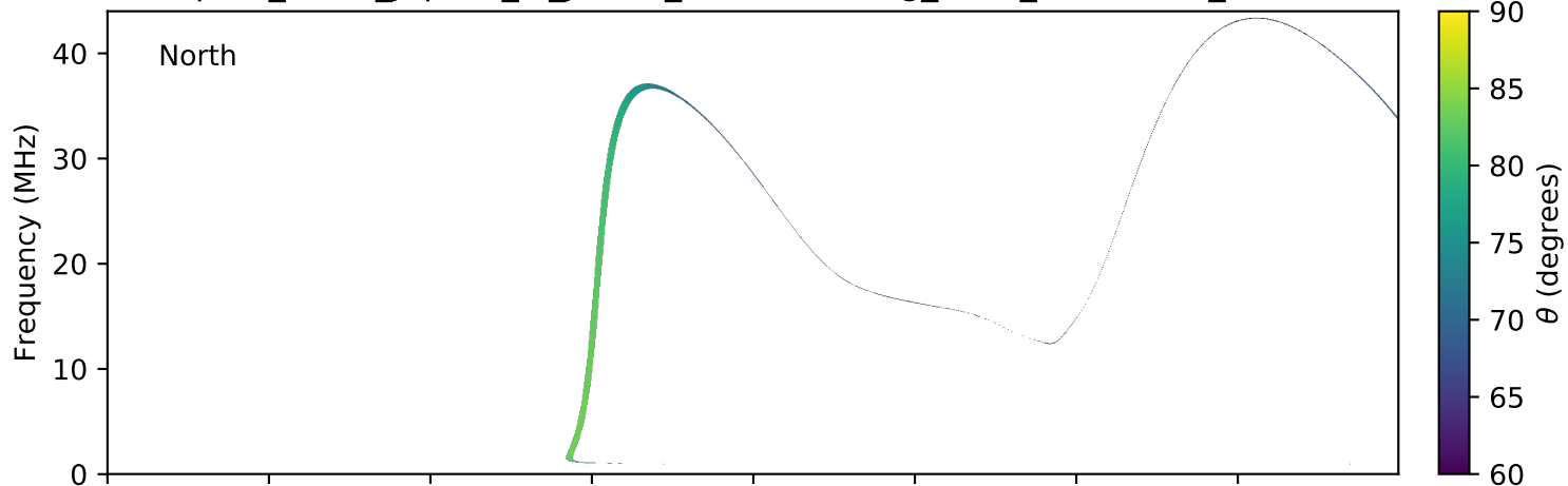
expres_earth_jupiter_io_jrm09_lossc-wid1deg_3kev_20160325_v01.cdf
