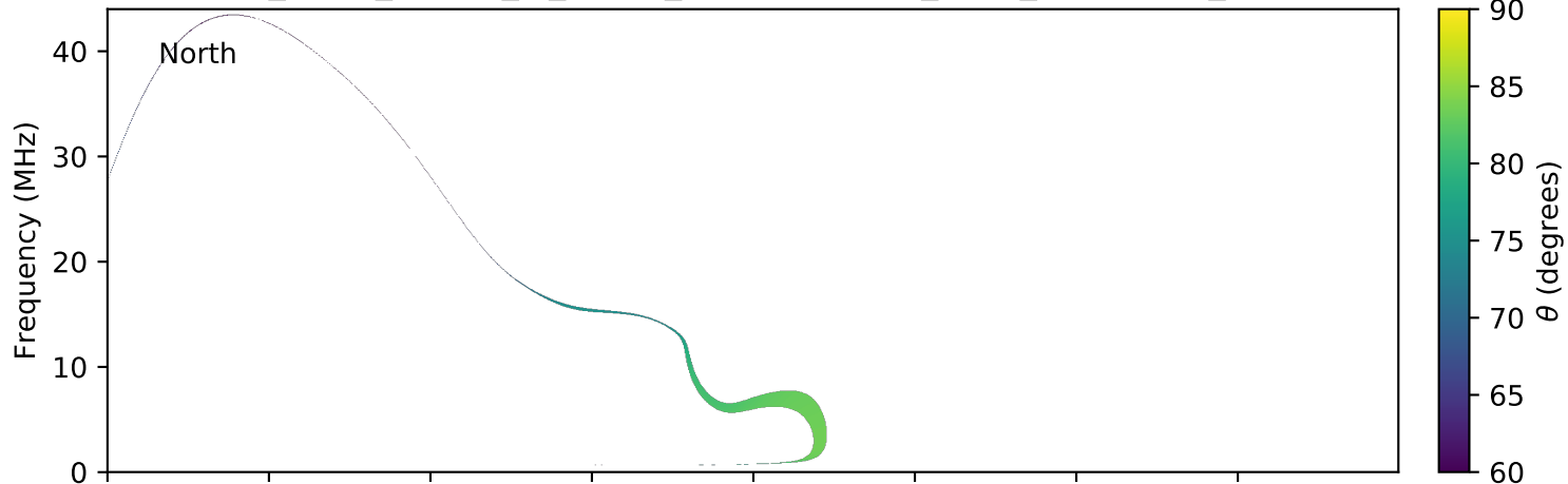
expres_earth_jupiter_io_jrm09_lossc-wid1deg_3kev_20160315_v01.cdf
