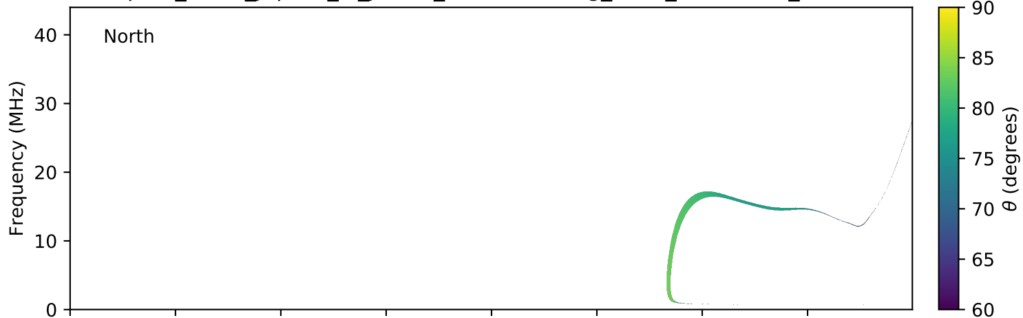
expres_earth_jupiter_io_jrm09_lossc-wid1deg_3kev_20160314_v01.cdf
