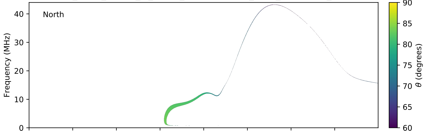
expres_earth_jupiter_io_jrm09_lossc-wid1deg_3kev_20160309_v01.cdf
