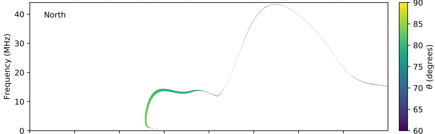
expres_earth_jupiter_io_jrm09_lossc-wid1deg_3kev_20160302_v01.cdf
