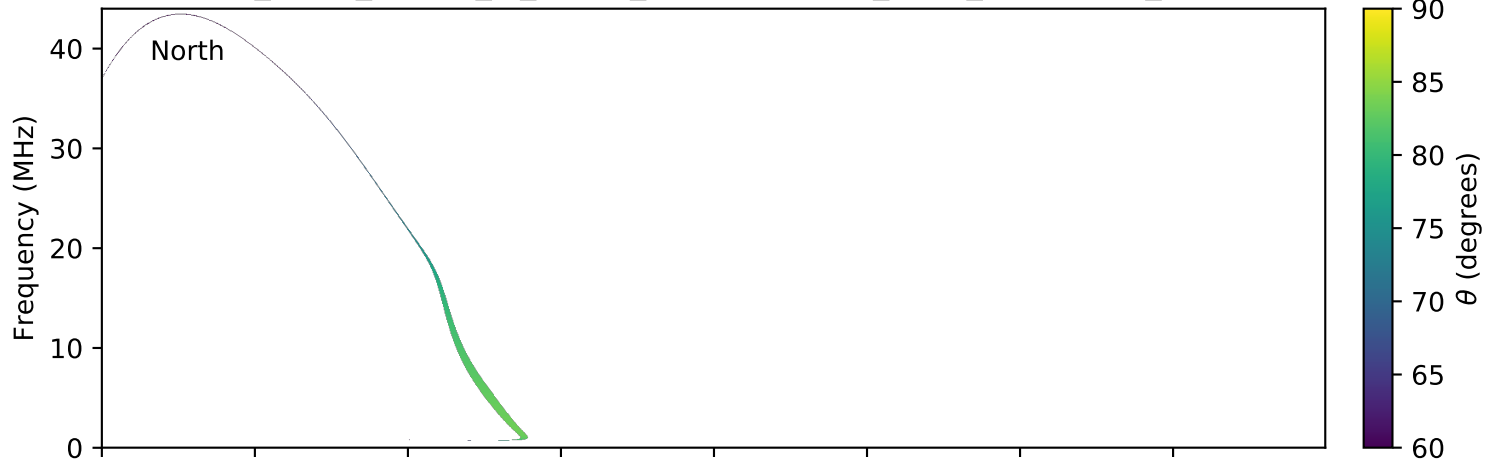
expres_earth_jupiter_io_jrm09_lossc-wid1deg_3kev_20160301_v01.cdf
