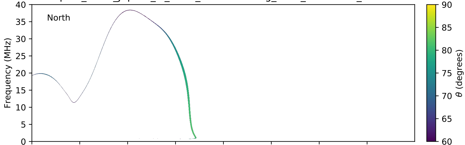
expres_earth_jupiter_io_isaac_lossc-wid1deg_5kev_20160331_v01.cdf
