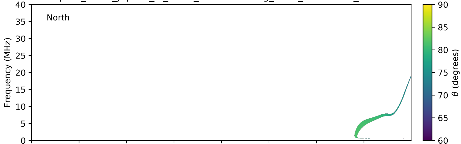
expres_earth_jupiter_io_isaac_lossc-wid1deg_5kev_20160328_v01.cdf
