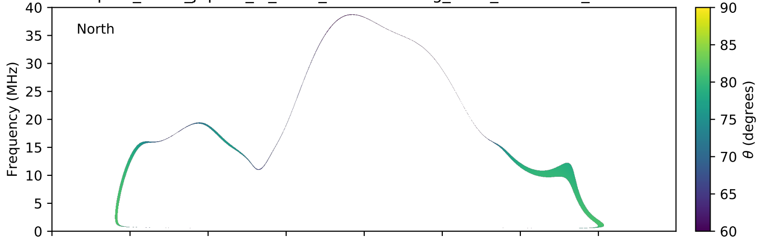
expres_earth_jupiter_io_isaac_lossc-wid1deg_5kev_20160327_v01.cdf
