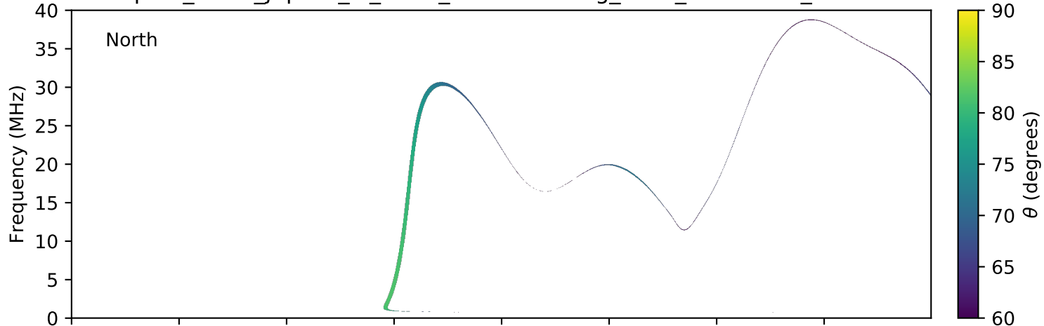
expres_earth_jupiter_io_isaac_lossc-wid1deg_5kev_20160325_v01.cdf
