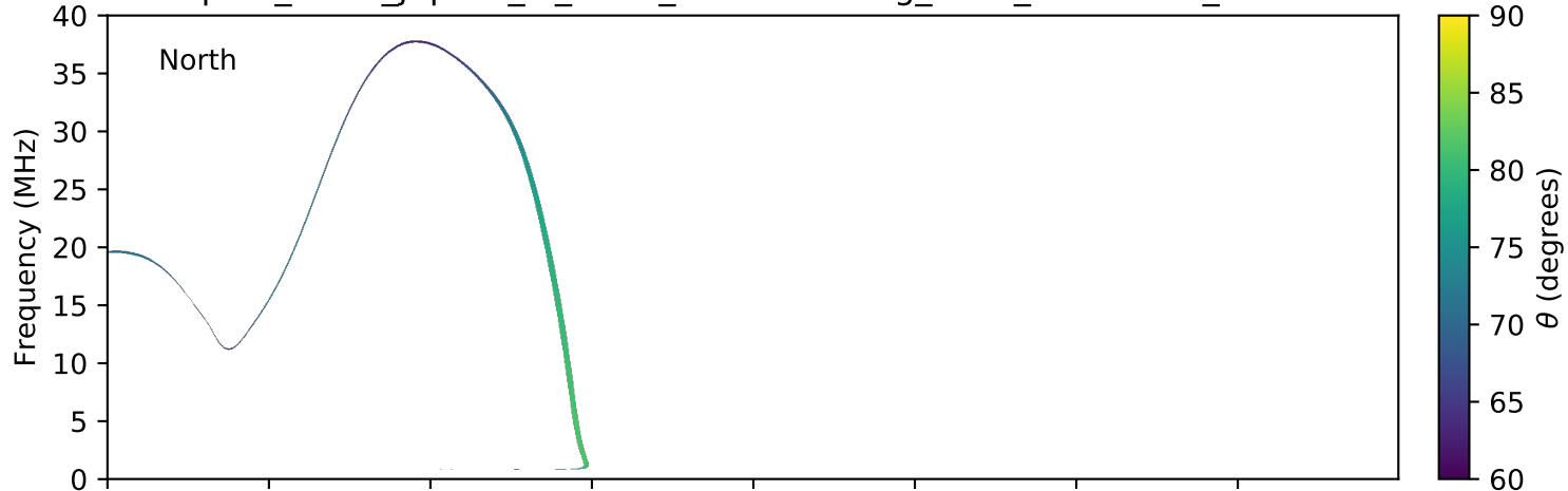
expres_earth_jupiter_io_isaac_lossc-wid1deg_5kev_20160324_v01.cdf
