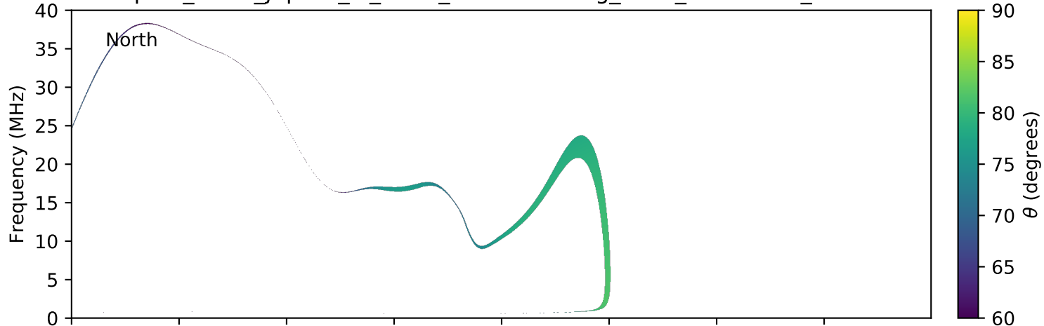
expres_earth_jupiter_io_isaac_lossc-wid1deg_5kev_20160322_v01.cdf
