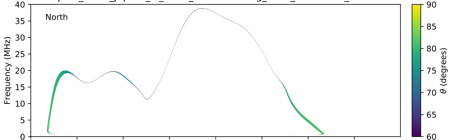
expres_earth_jupiter_io_isaac_lossc-wid1deg_5kev_20160320_v01.cdf
