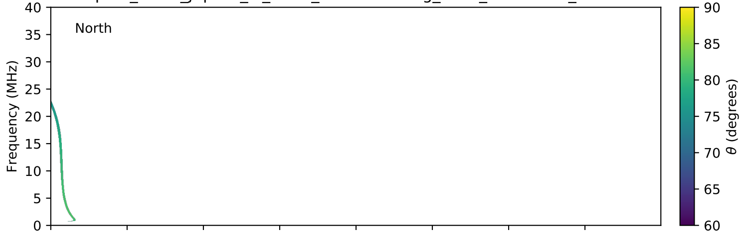
expres_earth_jupiter_io_isaac_lossc-wid1deg_5kev_20160319_v01.cdf
