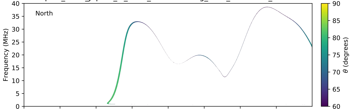
expres_earth_jupiter_io_isaac_lossc-wid1deg_5kev_20160318_v01.cdf
