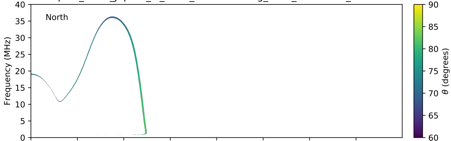
expres_earth_jupiter_io_isaac_lossc-wid1deg_5kev_20160317_v01.cdf
