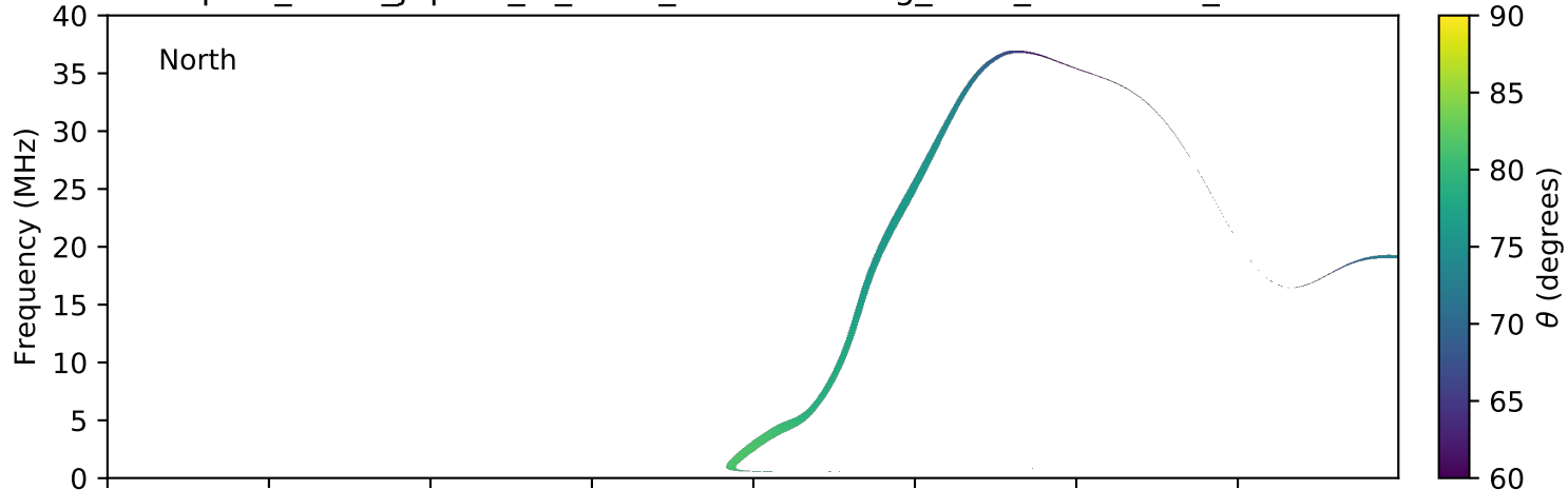
expres_earth_jupiter_io_isaac_lossc-wid1deg_5kev_20160316_v01.cdf
