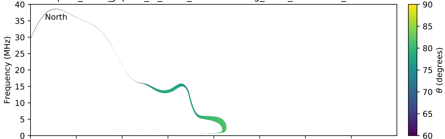
expres_earth_jupiter_io_isaac_lossc-wid1deg_5kev_20160315_v01.cdf
