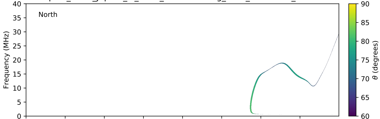
expres_earth_jupiter_io_isaac_lossc-wid1deg_5kev_20160314_v01.cdf
