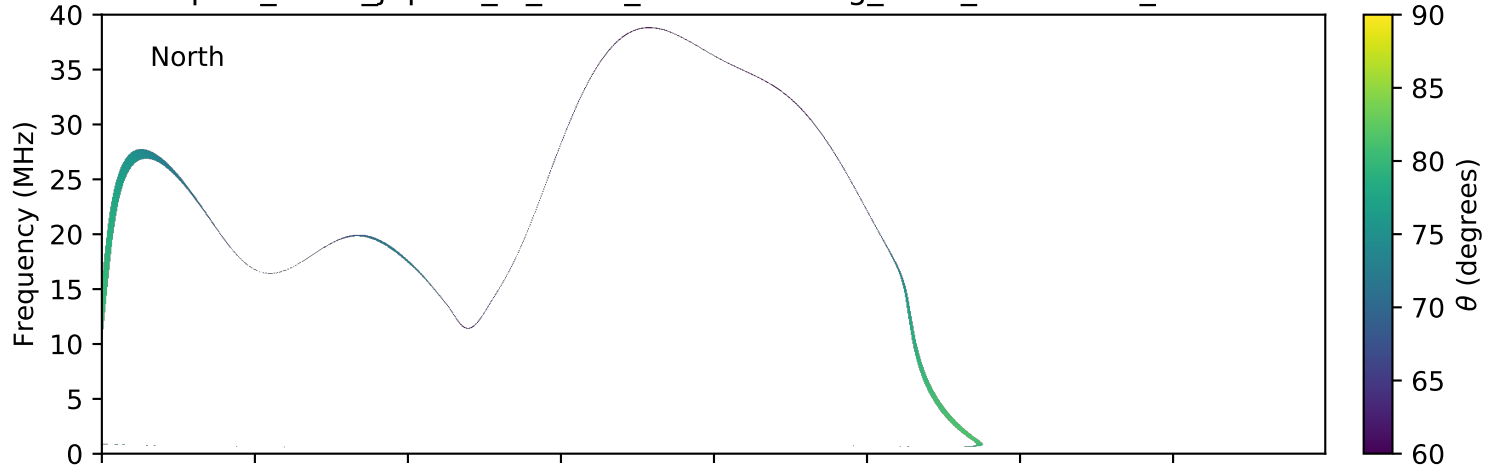
expres_earth_jupiter_io_isaac_lossc-wid1deg_5kev_20160313_v01.cdf
