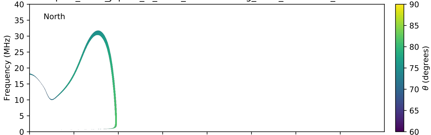
expres_earth_jupiter_io_isaac_lossc-wid1deg_5kev_20160310_v01.cdf
