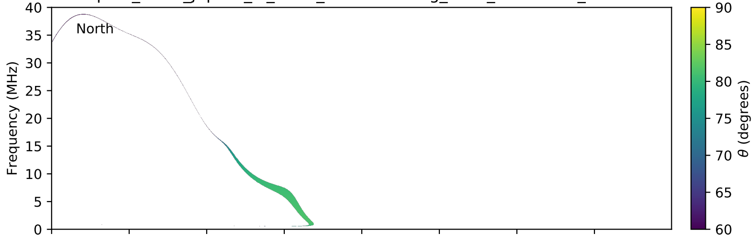
expres_earth_jupiter_io_isaac_lossc-wid1deg_5kev_20160308_v01.cdf
