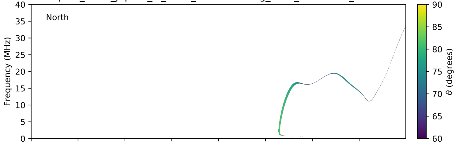
expres_earth_jupiter_io_isaac_lossc-wid1deg_5kev_20160307_v01.cdf
