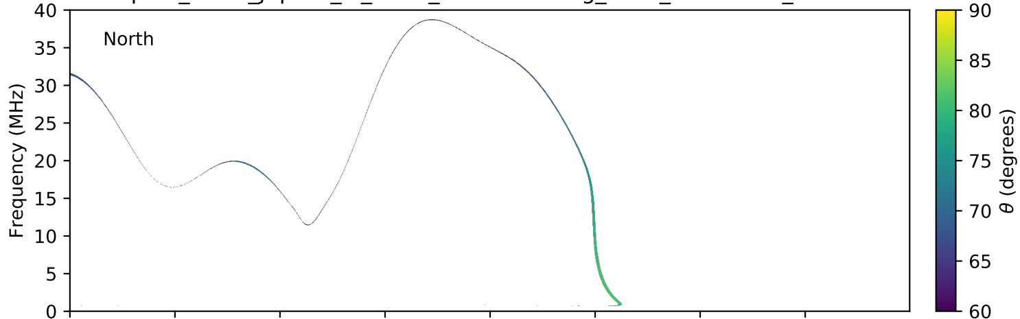
expres_earth_jupiter_io_isaac_lossc-wid1deg_5kev_20160306_v01.cdf
