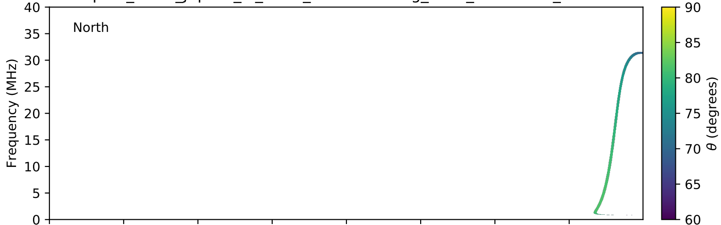
expres_earth_jupiter_io_isaac_lossc-wid1deg_5kev_20160305_v01.cdf
