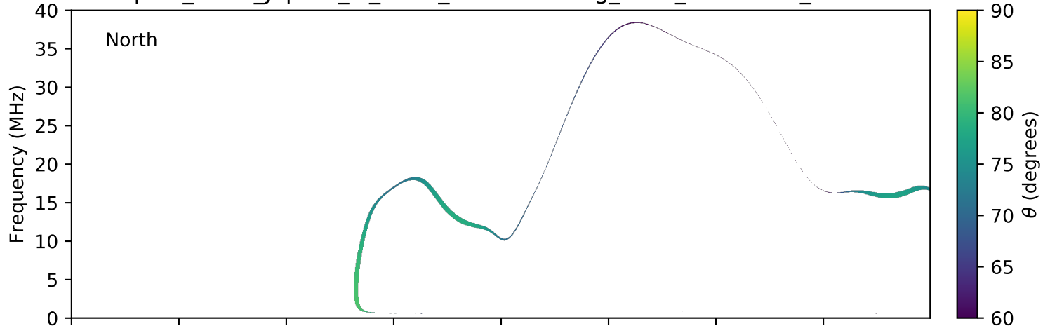
expres_earth_jupiter_io_isaac_lossc-wid1deg_5kev_20160302_v01.cdf
