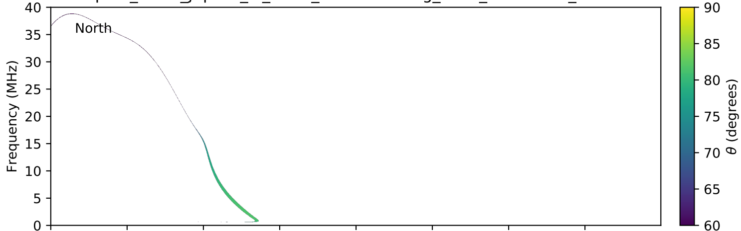
expres_earth_jupiter_io_isaac_lossc-wid1deg_5kev_20160301_v01.cdf
