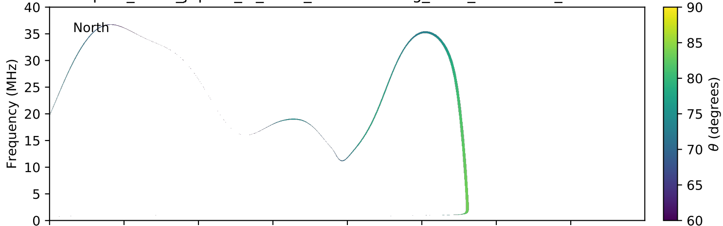
expres_earth_jupiter_io_isaac_lossc-wid1deg_3kev_20160329_v01.cdf
