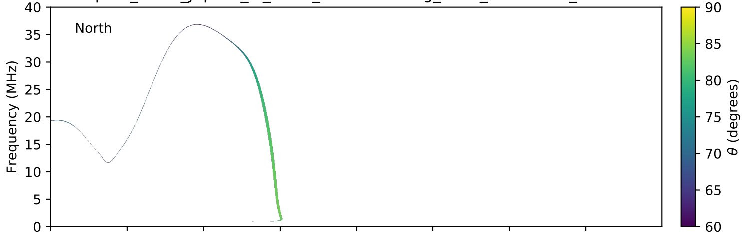
expres_earth_jupiter_io_isaac_lossc-wid1deg_3kev_20160324_v01.cdf
