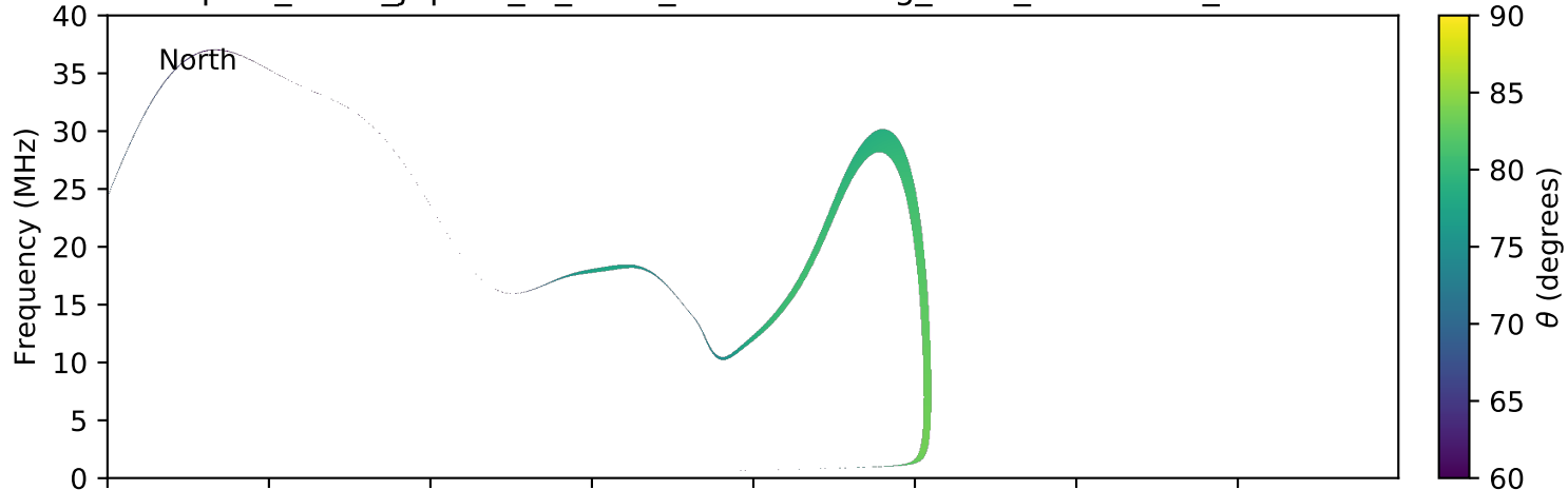
expres_earth_jupiter_io_isaac_lossc-wid1deg_3kev_20160322_v01.cdf
