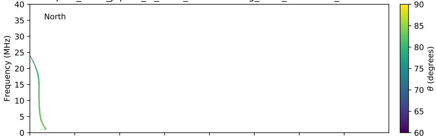
expres_earth_jupiter_io_isaac_lossc-wid1deg_3kev_20160319_v01.cdf
