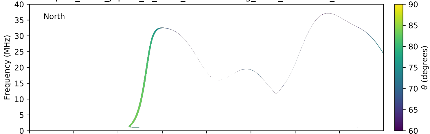
expres_earth_jupiter_io_isaac_lossc-wid1deg_3kev_20160318_v01.cdf
