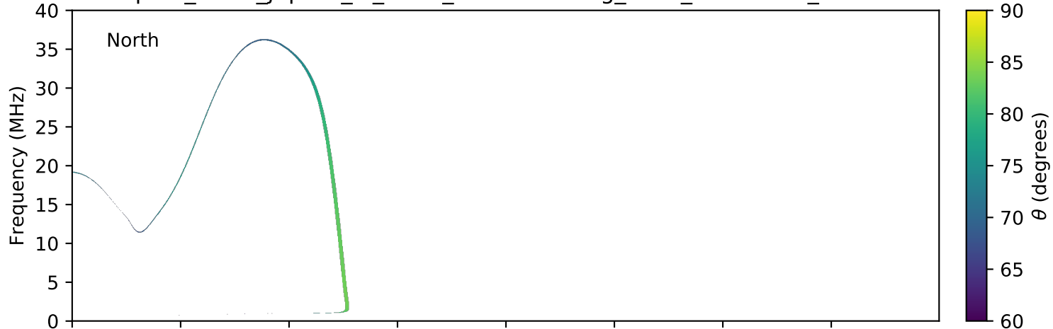
expres_earth_jupiter_io_isaac_lossc-wid1deg_3kev_20160317_v01.cdf
